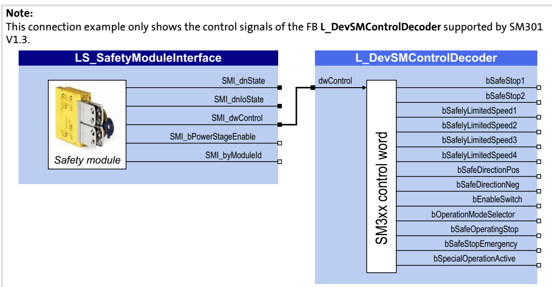
[2-4] Example: Decoding of the SMI_dwControl control signal into individual boolean control signals
