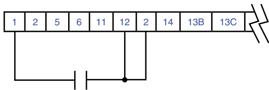
Run/Stop Contact
